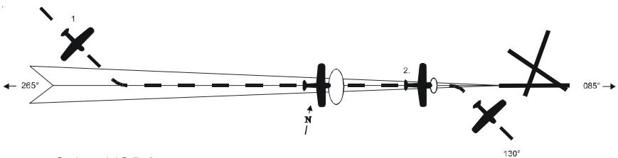
Fig. 3-29. AP Display, NAV Mode Engaged, Track VOR Front Course Inbound
