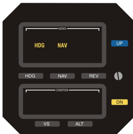
Fig. 3-6. AP Display, HDG Mode Engaged, NAV Mode Armed
